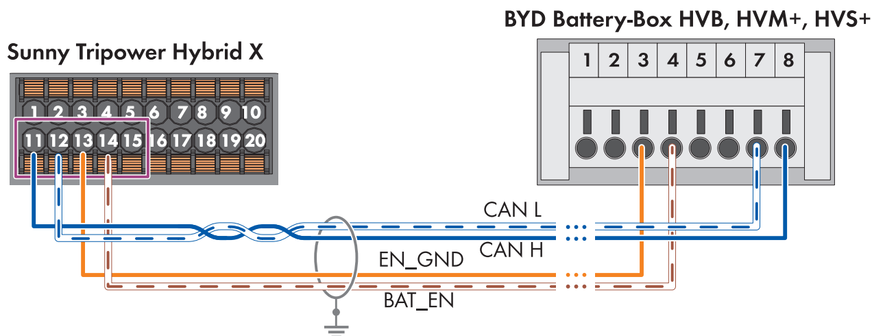
Figure 2: Cabling plan for the circuitry of Sunny Tripower Hybrid X with BYD Battery-Box HVB, HVM+ and HVS+. The individual cable ends must be provided with a 12 mm long bootlace ferrule.
