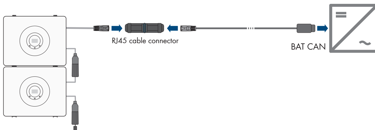
Figure 1: Cabling plan Sunny Tripower Hybrid X with SMA Home Storage
