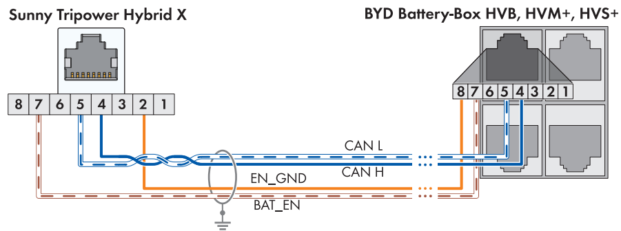
Figure 3: Cabling plan: Sunny Tripower Hybrid X with BYD Battery-Box HVB, HVM+ and HVS+.
